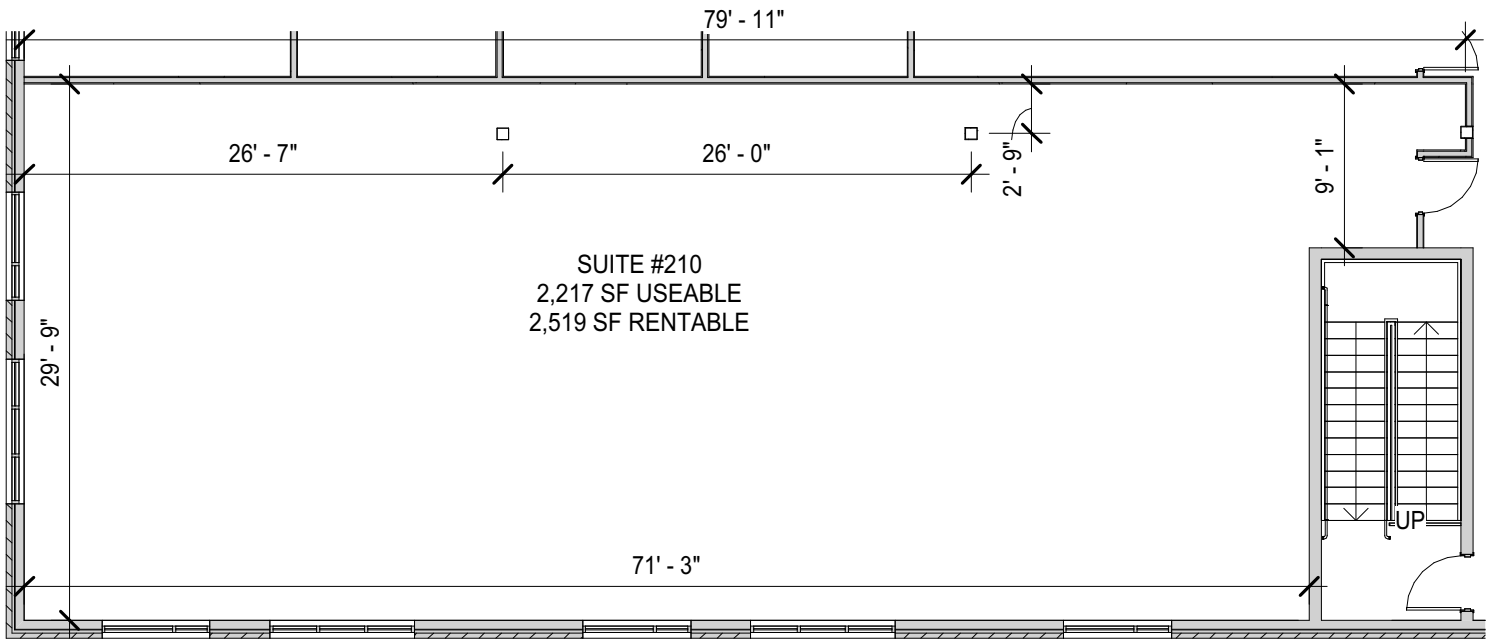
SUITE #210 FLOOR PLAN
