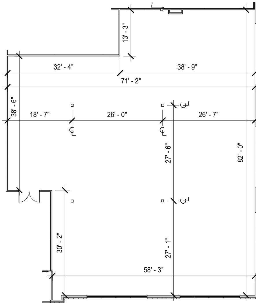
SUITE #110 FLOOR PLAN
