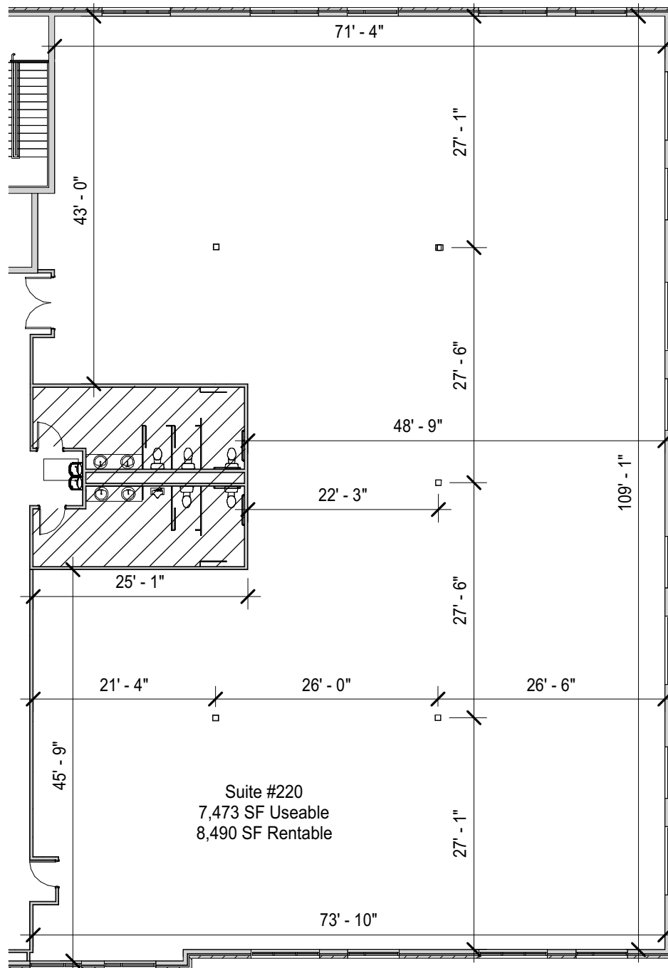
SUITE #220 FLOOR PLAN
